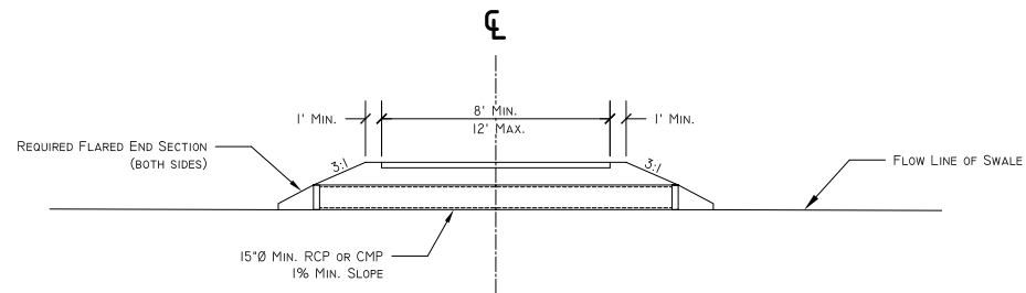
CROSS-SECTION
