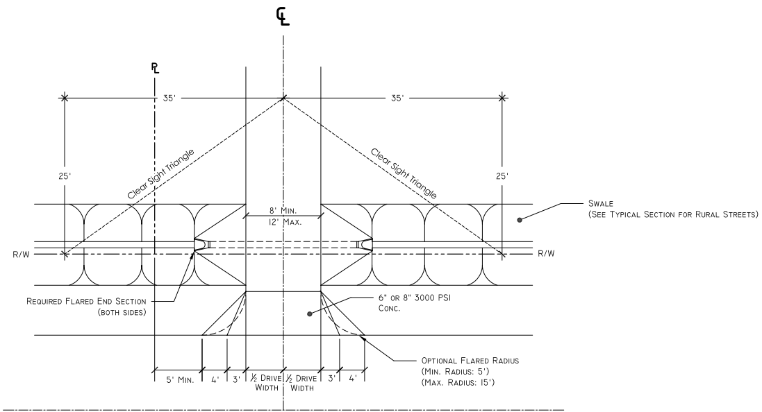
PLAN VIEW
